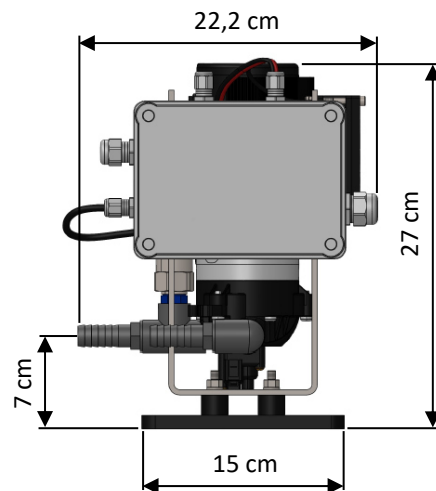
PUMP GROUP
