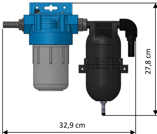
5 MICRON FILTER GROUP
