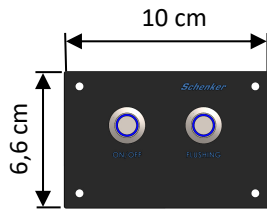
CONTROL PANEL
