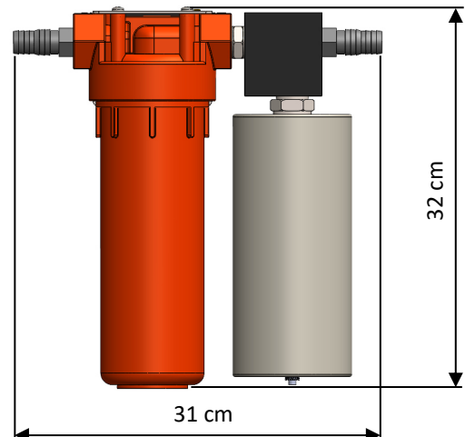
5 MICRON FILTER GROUP Depth: 11,3 cm
