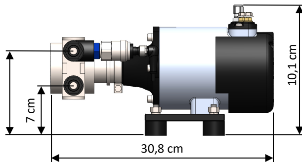
PUMP GROUP Depth: 25,5 cm - Weight: 6,7 kg
