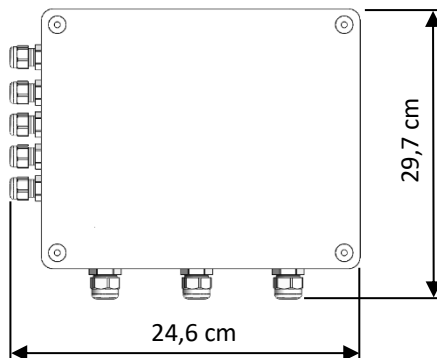
ELECTRICAL PUMP BOX Depth: 12,8 cm
