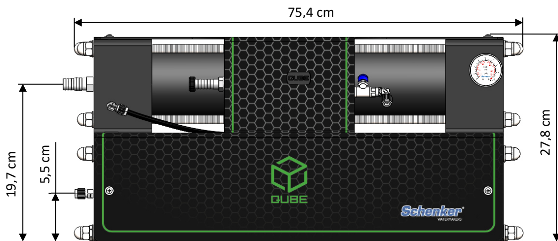
WATERMAKER Depth: 33,6 cm - Weight: 42,2 kg
