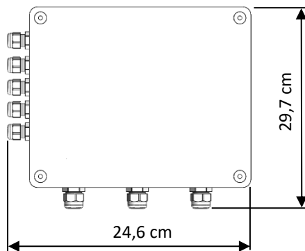
ELECTRICAL PUMP BOX (BASIC) Depth: 12,8 cm
