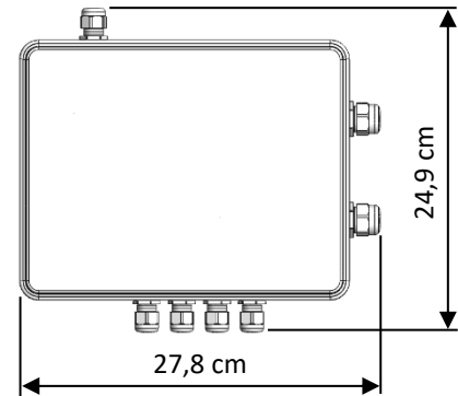
ELECTRICAL PUMP BOX (TOUCH) Depth: 9,6 cm
