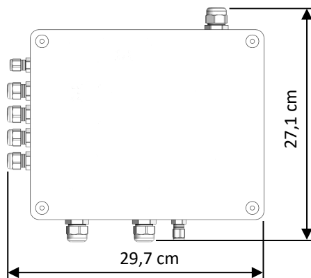
ELECTRICAL PUMP BOX (BASIC) Depth: 12,8 cm
