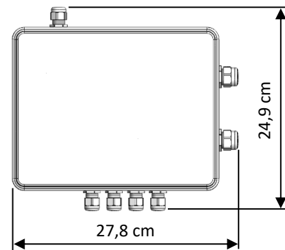
ELECTRICAL PUMP BOX (TOUCH) Depth: 9,6 cm
