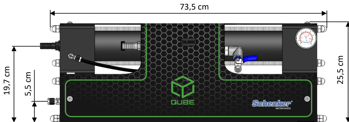
WATERMAKER Depth: 19,4 cm - Weight: 22,9 kg
