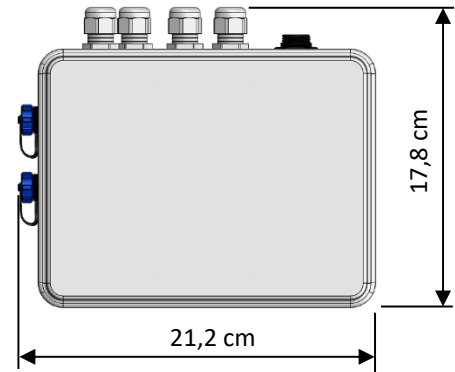
COMPUTER BOX (TOUCH) Depth: 8 cm
