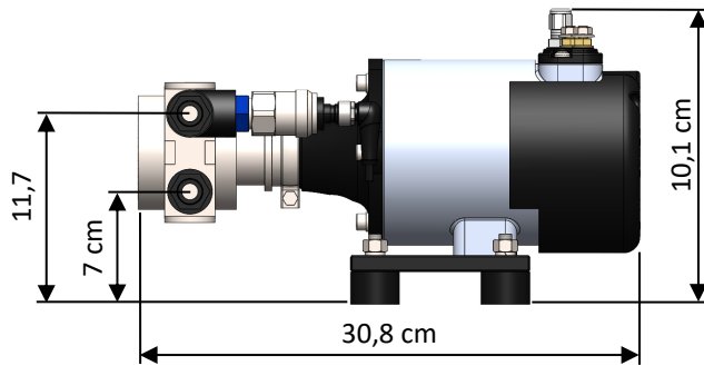
PUMP GROUP Depth: 25,5 cm - Weight: 6,7 kg
